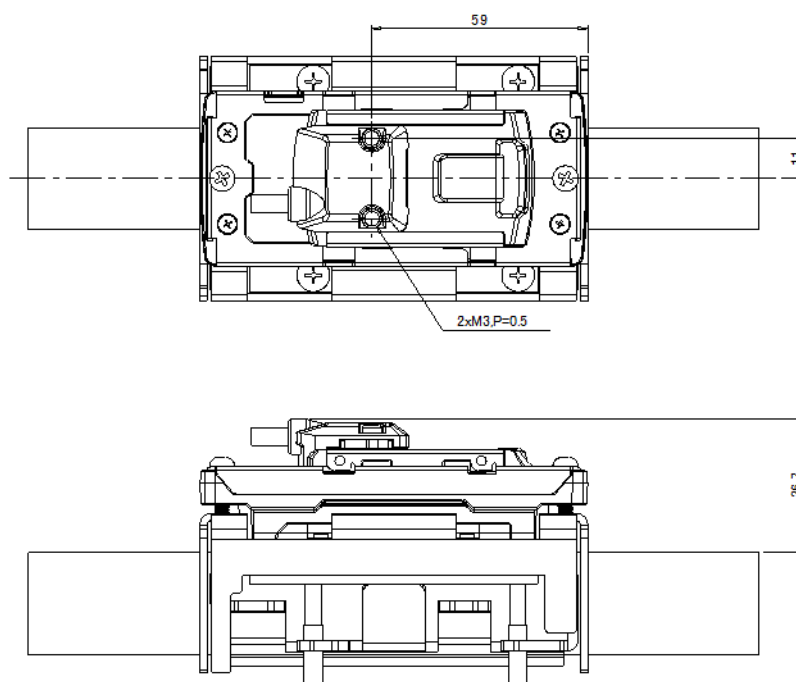
detection head
